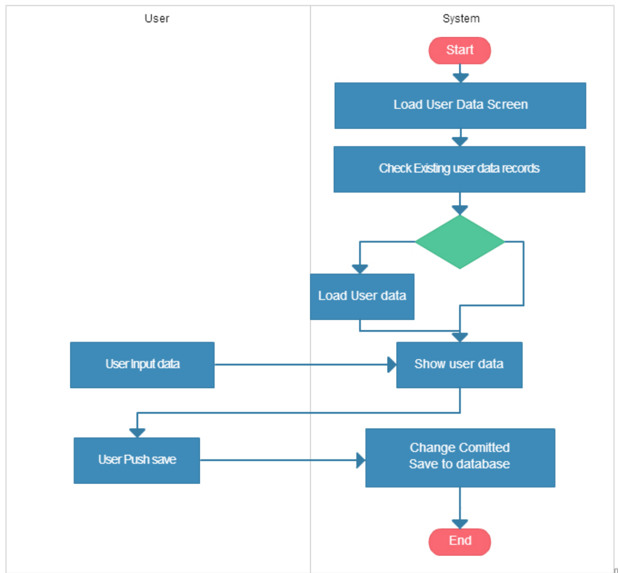
Figure 3.3 User data Swim lane diagram
