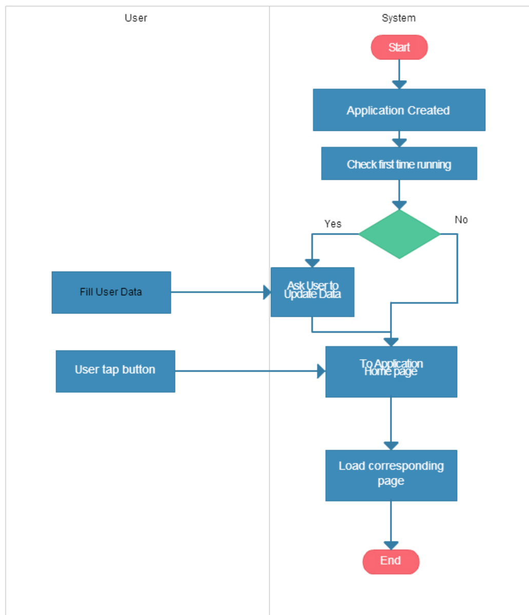
Figure 3.2 Main Activity swim lane diagram
